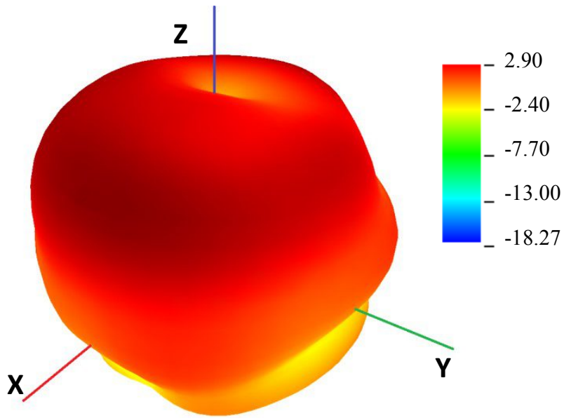
433 MHz Radiation pattern
