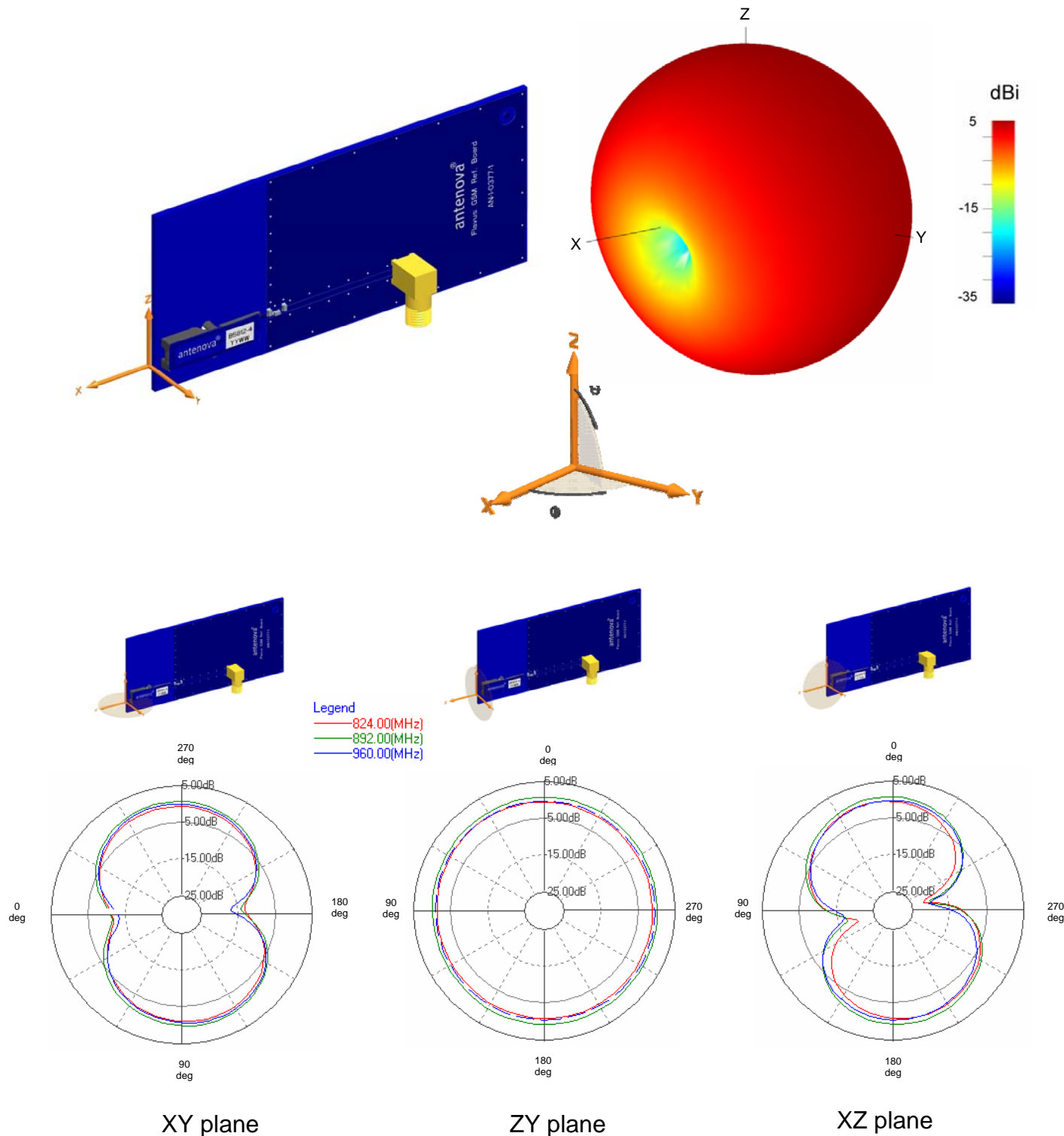
Patterns show combined polarisations measured on reference board 1020B5812-U1. 3D Pattern measured at 892MHz
