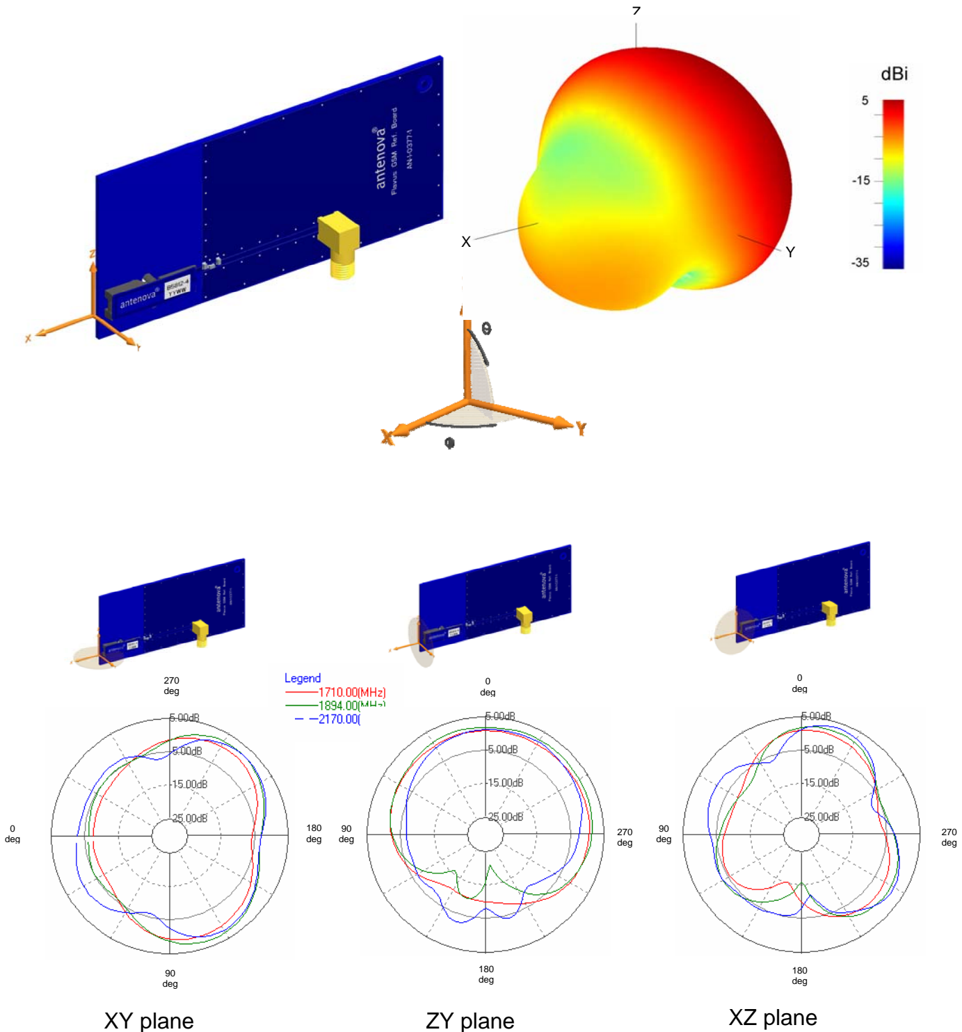
Patterns show combined polarisations measured on reference board 1020B5812-U1. 3D Pattern measured at 1894MHz
