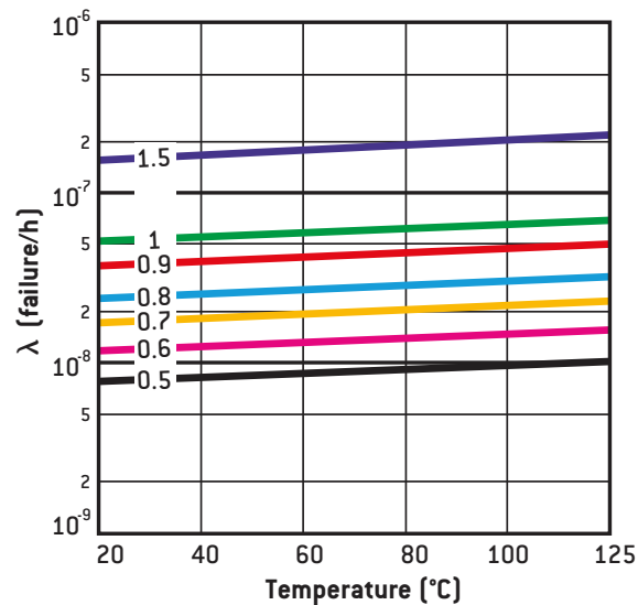
TYPICAL FAILURE RATE VERSUS TEMPERATURE
