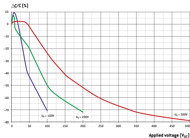
T DIELECTRIC: TYPICAL VOLTAGE COEFFICIENT AT 25°C (for all sizes)
