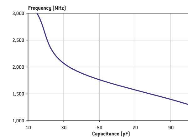
TYPICAL SERIES RESONANT FREQUENCY VERSUS CAPACITANCE
