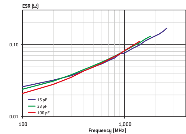
TYPICAL ESR VERSUS FREQUENCY
