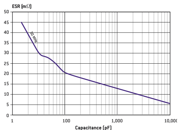
4040: TYPICAL ESR VERSUS CAPACITANCE
