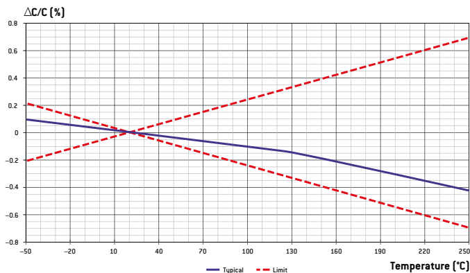
NPO: TYPICAL CAPACITANCE VARIATION VERSUS TEMPERATURE
