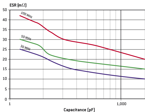
2225: TYPICAL ESR VERSUS CAPACITANCE
