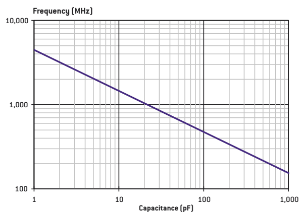
2225: TYPICAL SERIES RESONANT FREQUENCY VERSUS CAPACITANCE
