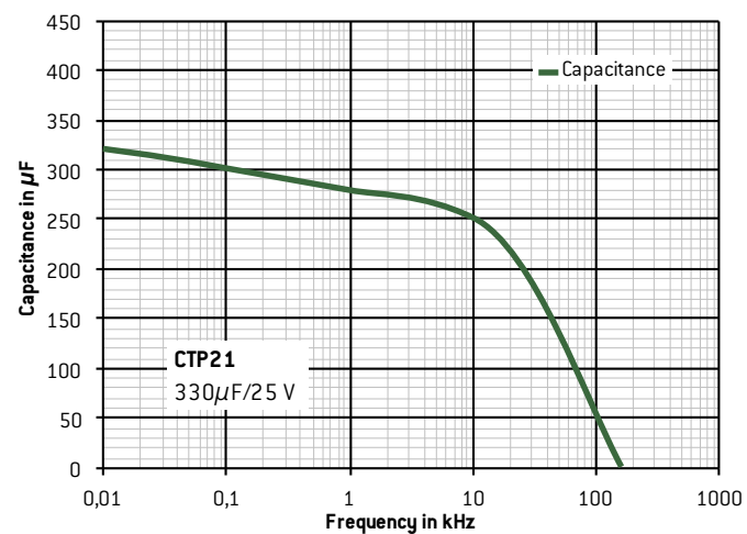
CAPACITANCE CHANGE VS FREQUENCY (TYPICAL)
