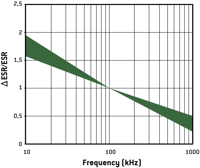
ESR CHANGE VS FREQUENCY
